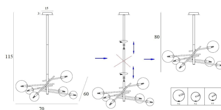
LOLLIPOP P0395 6 x max. 40W G9 230V
