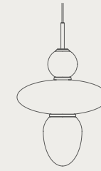
RIZZATTO 43 Dimensions \phi 400mm x 626mm Options satin brass / opal or satin silver / opal Cable colour gold or silver fabric Cable Length max 4000mm Light source E27
