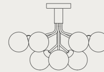
APIALES 9 CEILING Dimensions ø595mm x 399mm Glass dimensions ø120mm Options brushed brass / opal, satin black / opal, brushed brass / optic gold or satin black / optic smoked Light source G9
