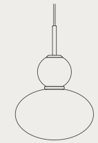
RIZZATTO 32 Dimensions \phi 300mm x 448mm Options satin brass / opal or satin silver / opal Cable colour gold or silver fabric Cable Length max 4000mm Light source E14
