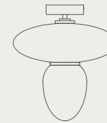
RIZZATTO 42 Dimensions \phi 400mm x 449mm Options satin brass / opal or satin silver / opal Light source E27
